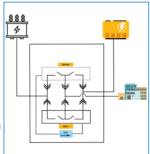
4) Tow Way Bypass Mechanism
