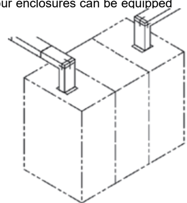
Automatic Transfer Switch Busway Flange Connection
